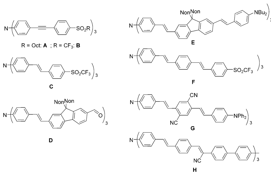
Scheme 3. Structures of reference compounds for comparison to literature chromophores: A , [25b] B , [25b,35] C , [26a] D , [26a] E , [26b] F , [26a] G , [36a] and H . [36b]
