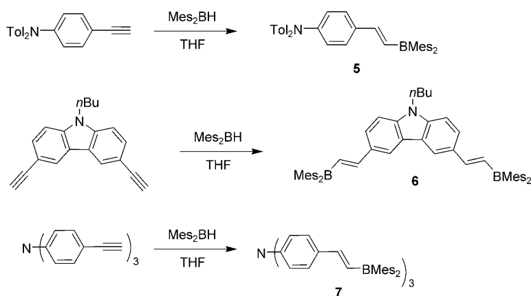
Scheme 2. Synthesis of chromophores 5–7 .
