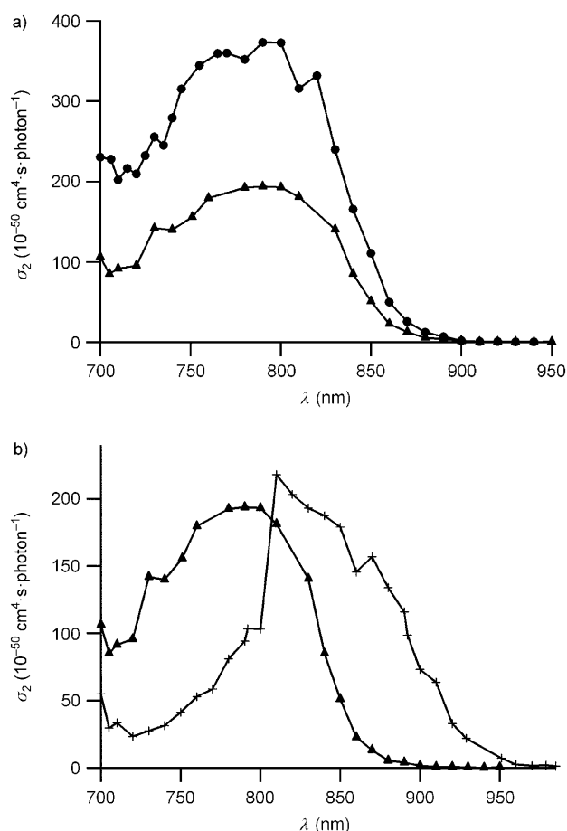
Figure 1. Comparison of TPA spectra in toluene of dipolar compounds: a) 1 (▲) and 2 (●): length effect and b) 1 (▲) and 5 (+): connector effect.
