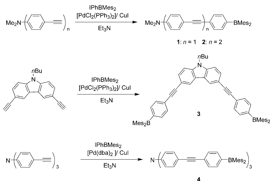
Scheme 1. Synthesis of chromophores 1–4 .
