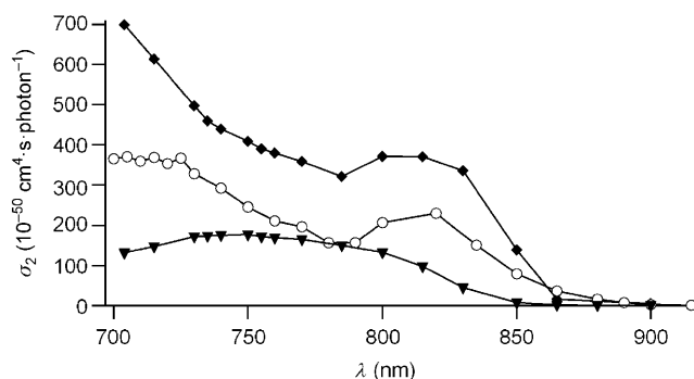
Figure 3. Comparison of TPA spectra of compound 4 (○) with reference chromophores A [25b] (▼) and B [25b,35] (◆) in toluene: effect of the peripheral acceptor group.
