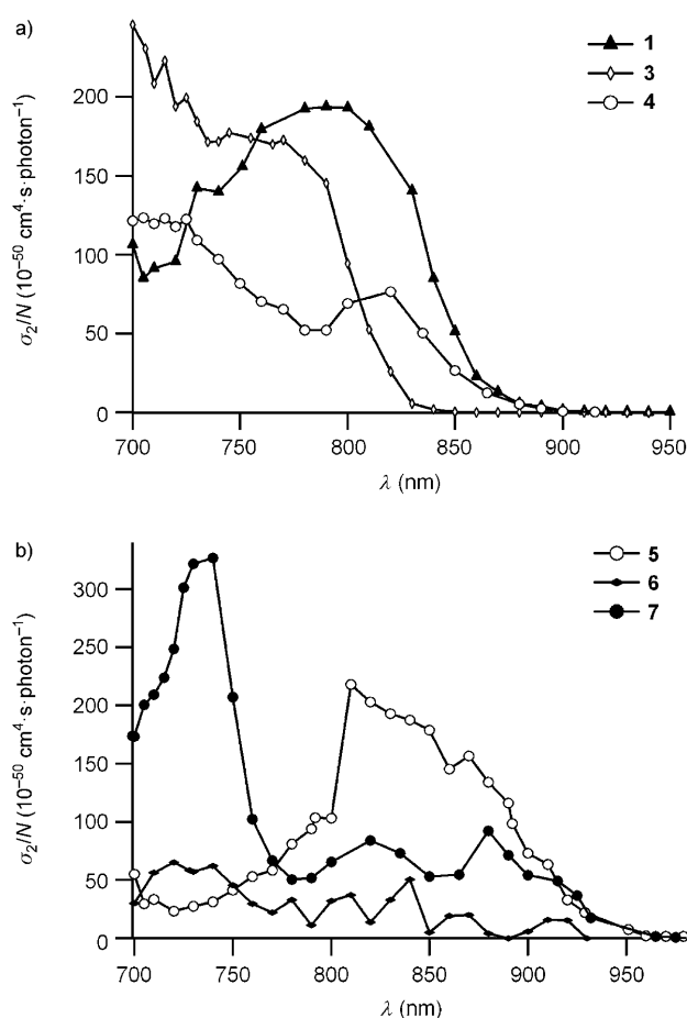
Figure 2. Comparison of the branching effect on TPA spectra normalised for the number of branches (N) in toluene: a) phenylethynyl-based chromophores 1 , 3 , 4 and b) vinylene-based compounds 5 , 6 and 7 .
